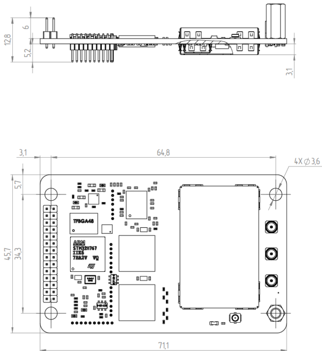
Figure 6.1– KV106 Board Layout and Dimensions
