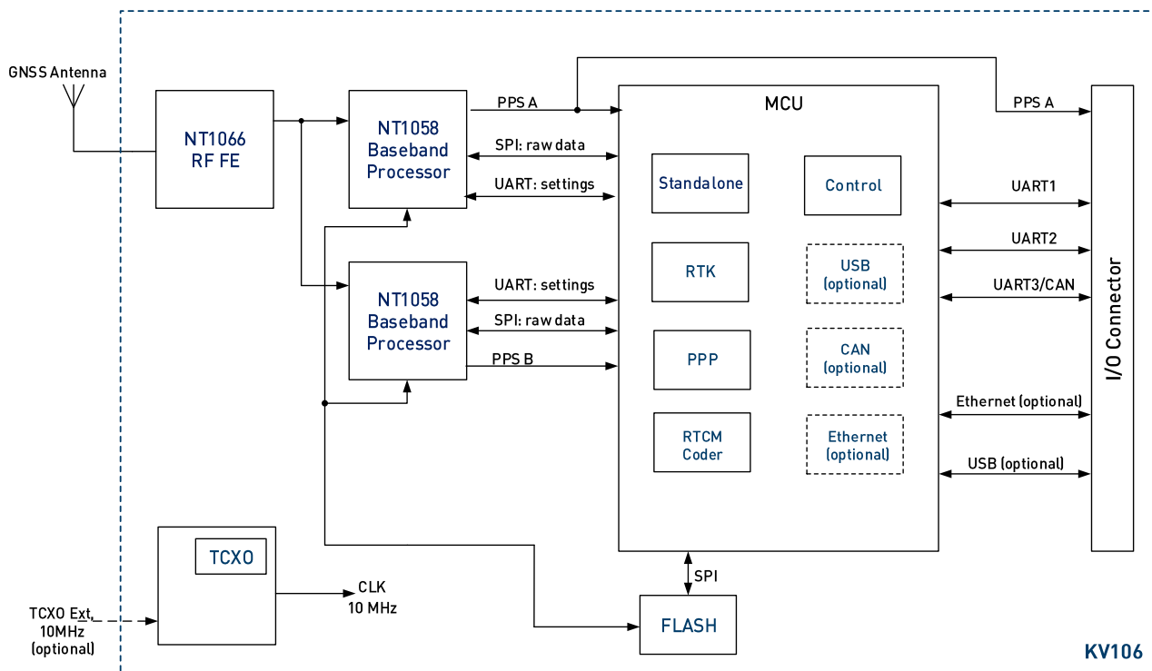
Figure 3.1– KV106 Block Diagram
