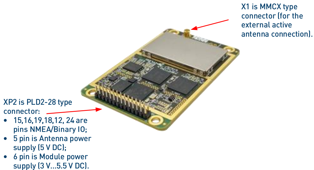
Figure 2.1– KV106 Top View 1
